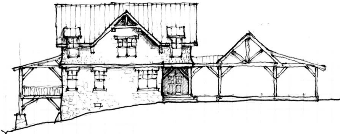
SIDE ELEVATION
