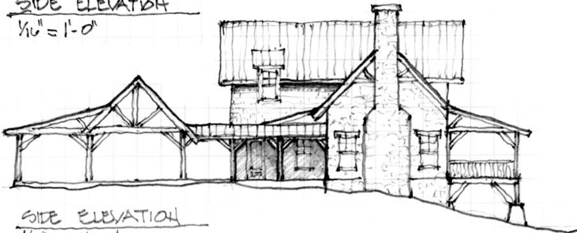
SIDE ELEVATION
