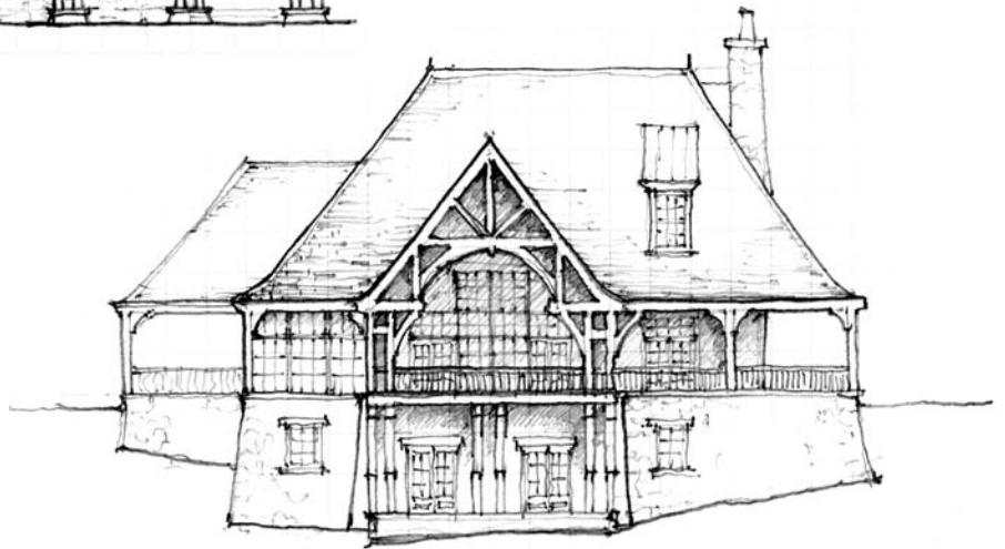
BACK ELEVATION
